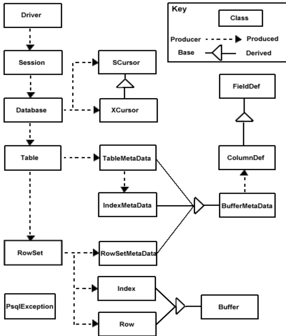
Figure 1 Java API Class Structure
